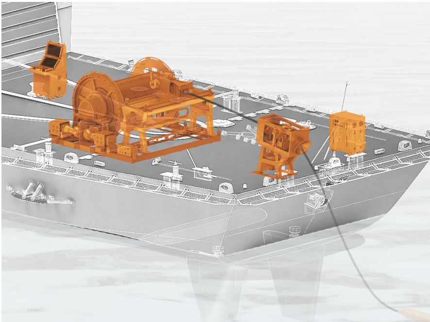
Hydraulic type of Winch system
